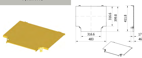
Horizontal T Cover P/N: A418
