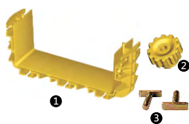
Coupler Kit A P/N: T5021
