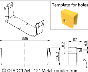
Fitting for Transitions Kit P/N: AD-OLPAN12x4
