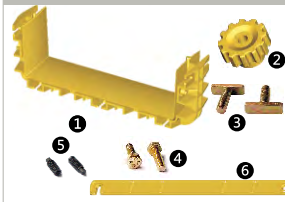
Coupler Kit B P/N: T4282
