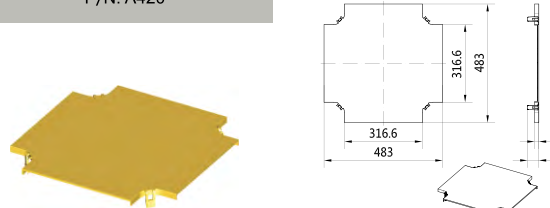
Horizontal Cross Cover P/N: A420
