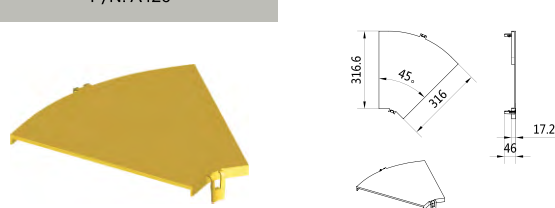
45° Horizontal Curve Cover P/N: A426
