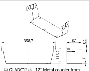
Fitting for Transitions Kit P/N: AD-OLADC12x4
