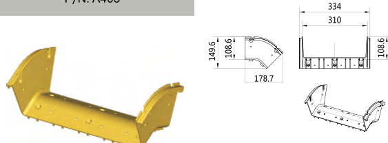
45° Down Curve P/N: A405
