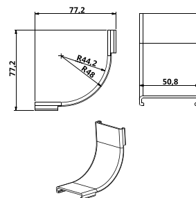
90° Down Curve Cover P/N: A118
