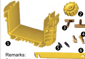
Coupler Kit B P/N: T3162
