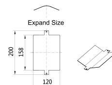
45° Up Curve Cover Kit P/N: T334
