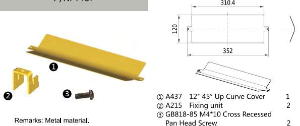
45° Up Curve Cover Kit P/N: T437
