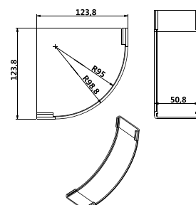
90° Up Curve Cover P/N: A116
