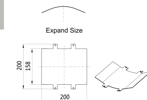
45° Down Curve Cover Kit P/N: T335
