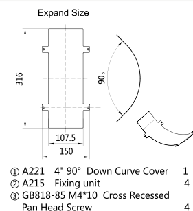
90° Down Curve Cover Kit P/N: T221
