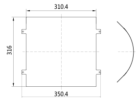
90° Down Curve Cover Kit P/N: T439
