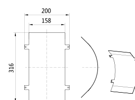
90° Down Curve Cover Kit P/N: T336
