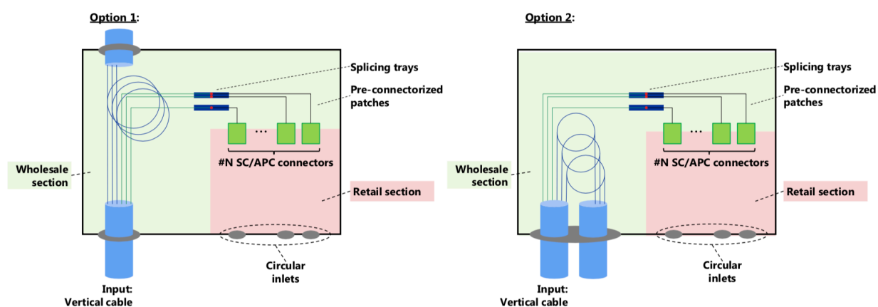
Figure 1 - FB Functional scheme
