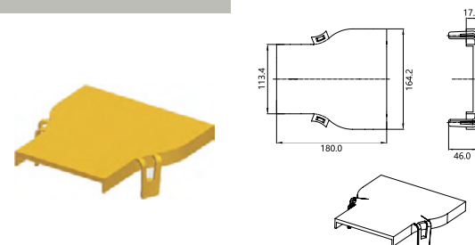
6" to 4" Adapter Cover P/N: A351
