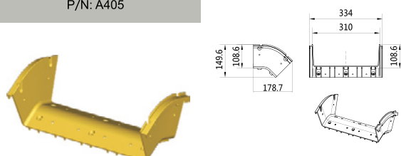
45° Down Curve P/N: A405
