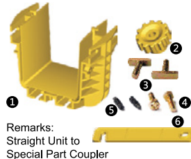
Coupler Kit B P/N: T2042
