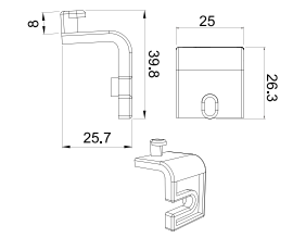
Vertical Cover Kit 4" P/N: T203
