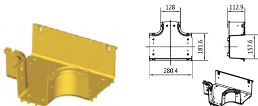
6" to 4" Horizontal T P/N: A320
