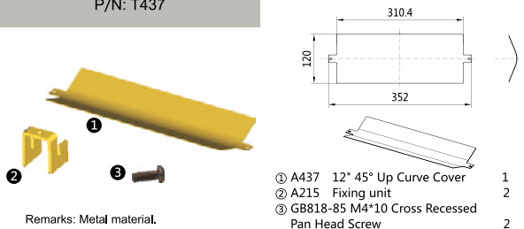
45° Up Curve Cover Kit P/N: T437
