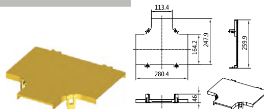
6" to 4" Horizontal T Cover P/N: A313
