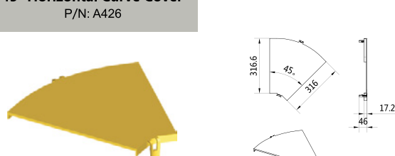
45° Horizontal Curve Cover P/N: A426
