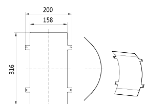
90° Down Curve Cover Kit P/N: T336
