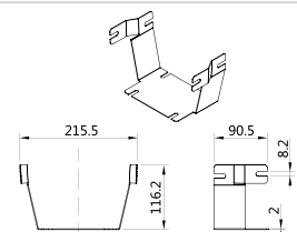
Fitting for Transitions Kit P/N: AD-OLADC6x4
