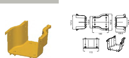
6" to 4" Adapter P/N: A350
