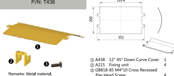
45° Down Curve Cover Kit P/N: T438
