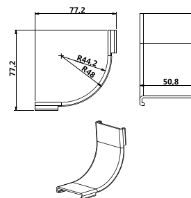
90° Down Curve Cover P/N: A118
