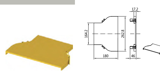
10" to 6" Adapter Cover P/N: A509
