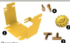
Fitting for Transitions Kit P/N: AD-OLPAN6X4
