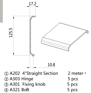
Straight Unit Cover Kit P/N: T202
