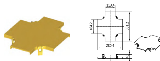
6" to 4" Horizontal Cross Cover P/N: A329
