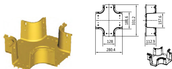
6" to 4" Horizontal Cross P/N: A326
