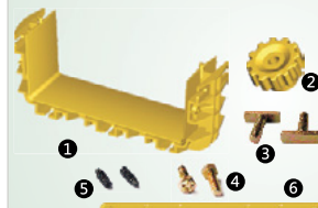
Coupler Kit B P/N: T5022
