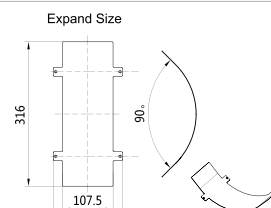
90° Down Curve Cover Kit P/N: T221
