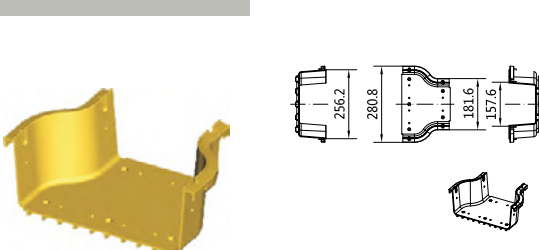
10" to 6" Adapter P/N: A505
